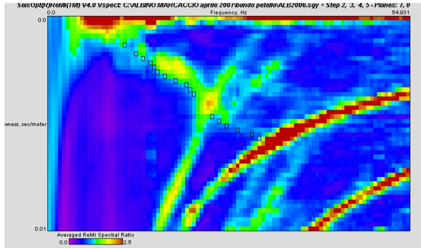
p-f Image with Dispersion Modeling Picks (fig. 1/b)
