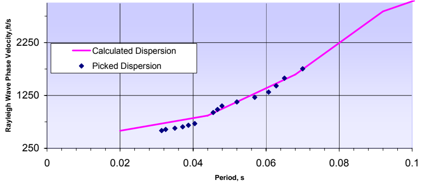
Dispersion Curve Showing Picks and Fit (fig. 1/a)
